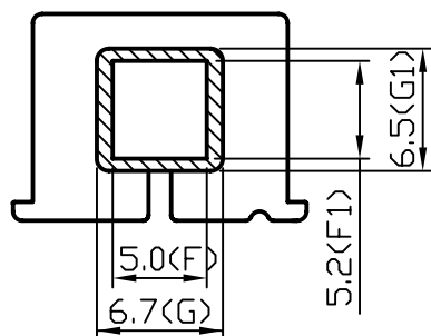
SECTION B-B/C-C
