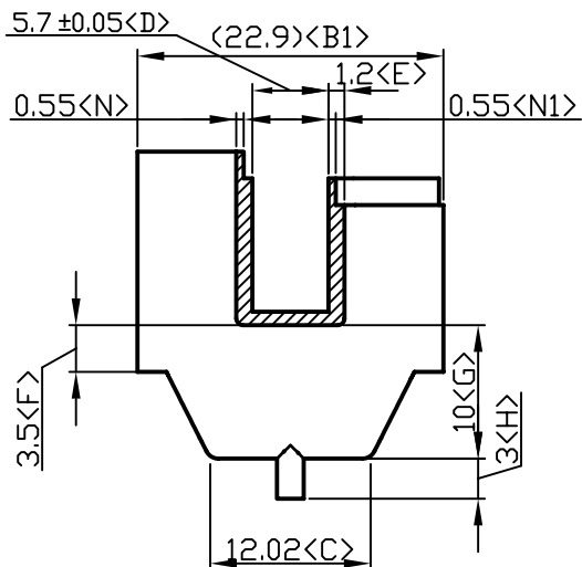
B-B VIEW
