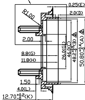
DETAIL D SECTION B-B
