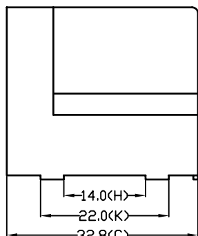
DETAIL D SCALE 2/1
