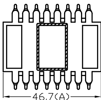
SECTION E-E
