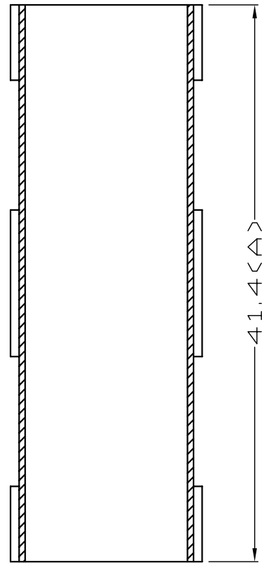
SECTION B-B
