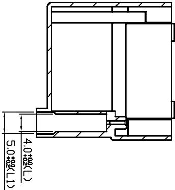
SECTION C-C
